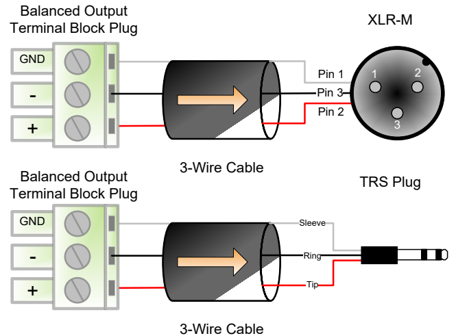
Figure 2 – Balanced Wiring Guide
