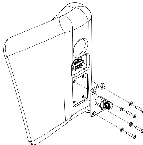
Figure 5.4: Bolt attachment
