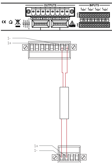
Figure 4.3: Bias Q1/Q2 output connection
