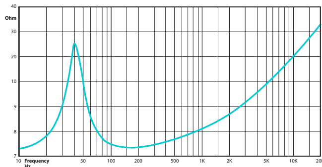
Impedance
