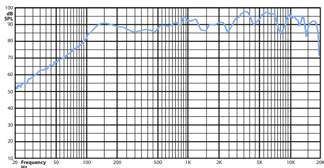
Frequency response
