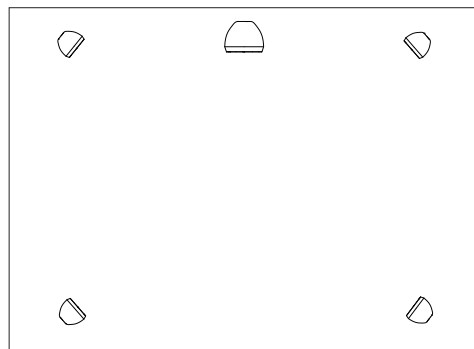
Figure 7.11: Loudspeaker layout
