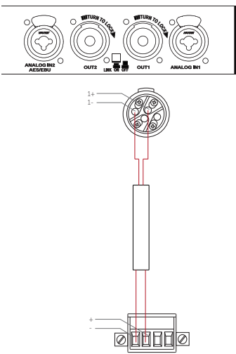
Figure 6.4: Bias V9
