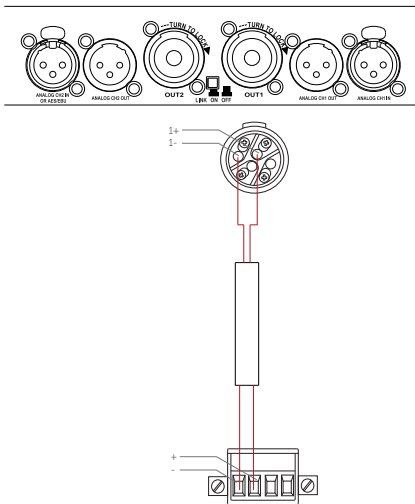
Figure 6.3: Bias V3
