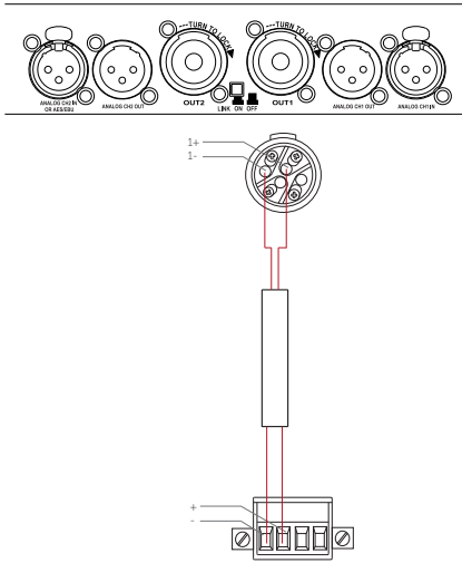
Figure 6.10: Bias V3
