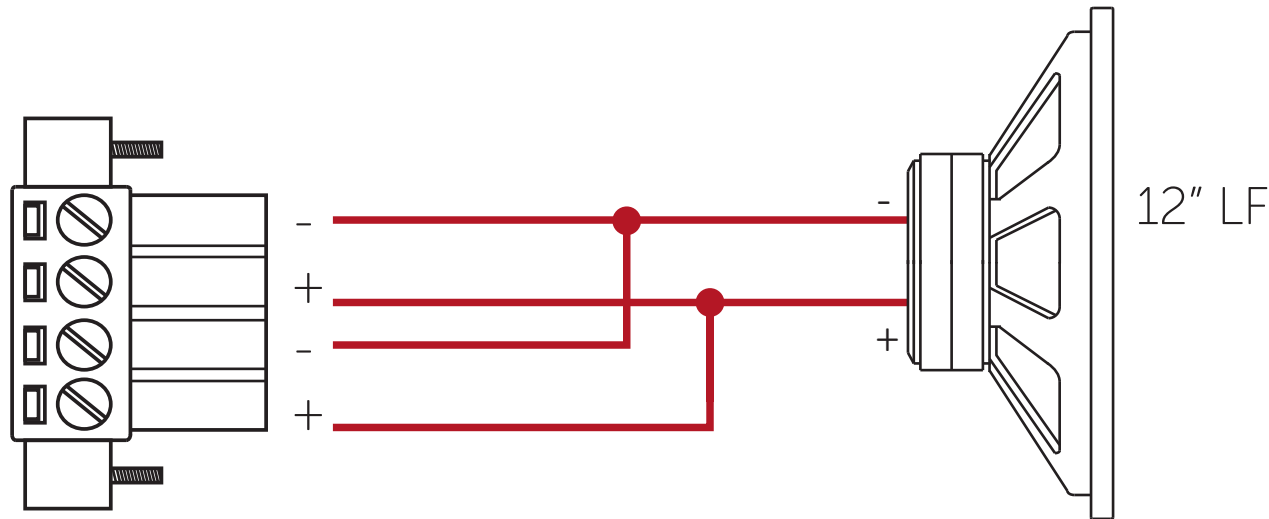
Figure 6.9: Indigo Sub wiring diagram
