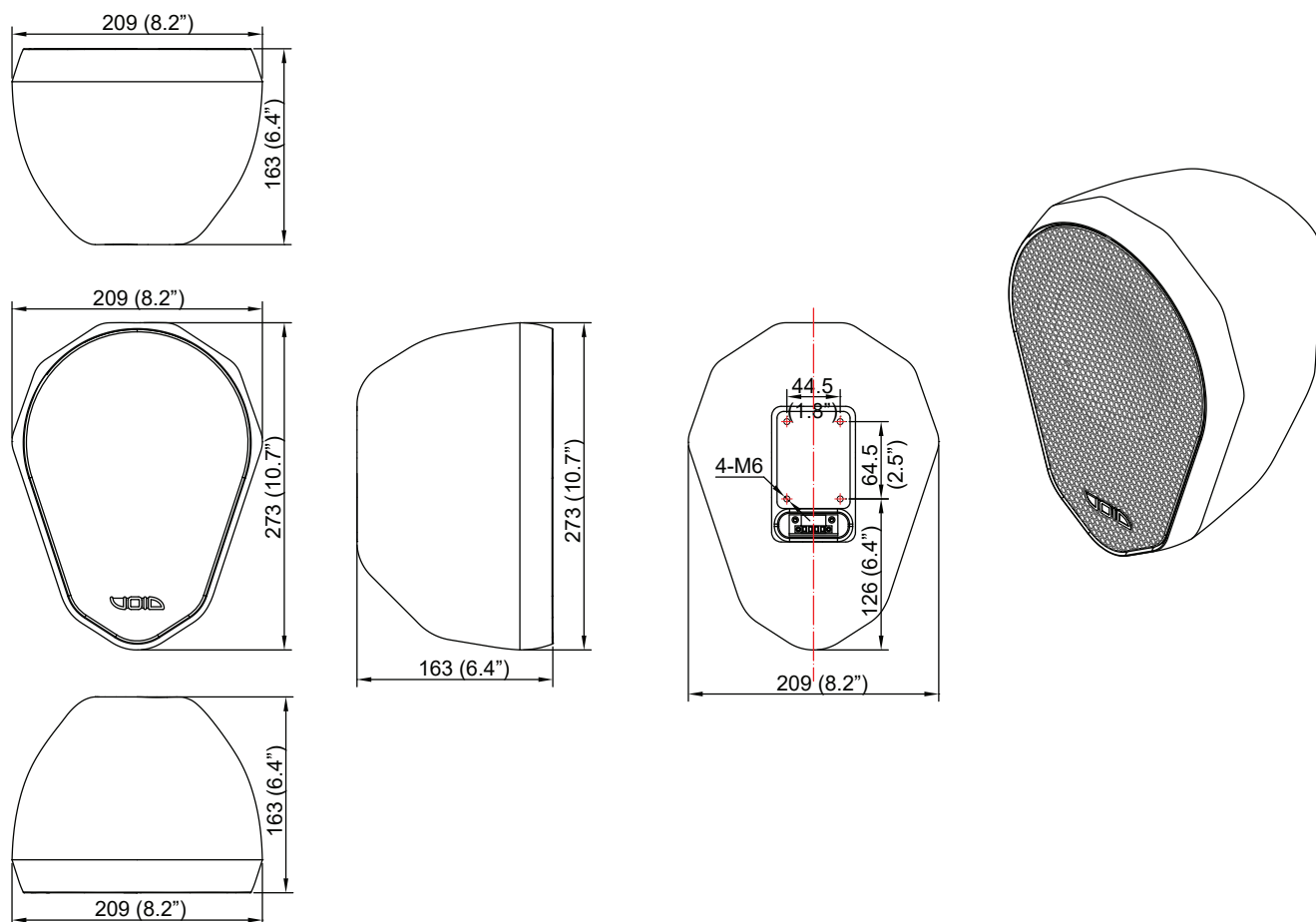
Figure 5.6: Dimensions
