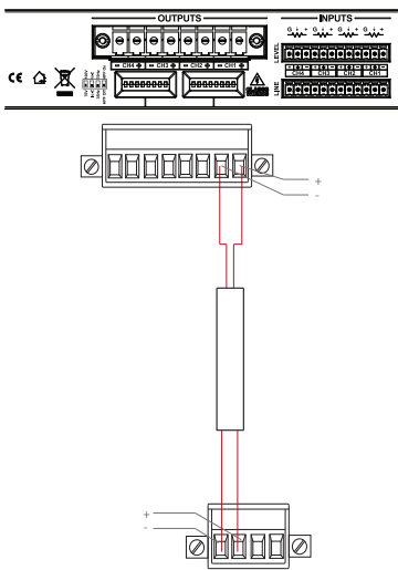
Figure 6.7: Bias Q2
