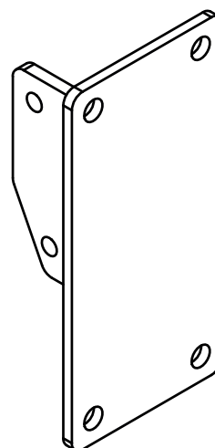
Figure 8.14: Rear bracket assembly
