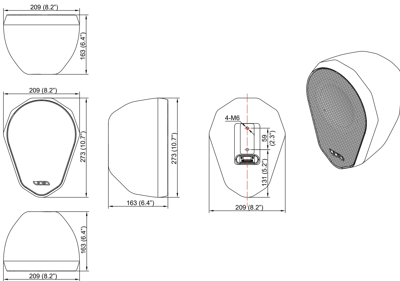
Figure 5.3: Dimensions
