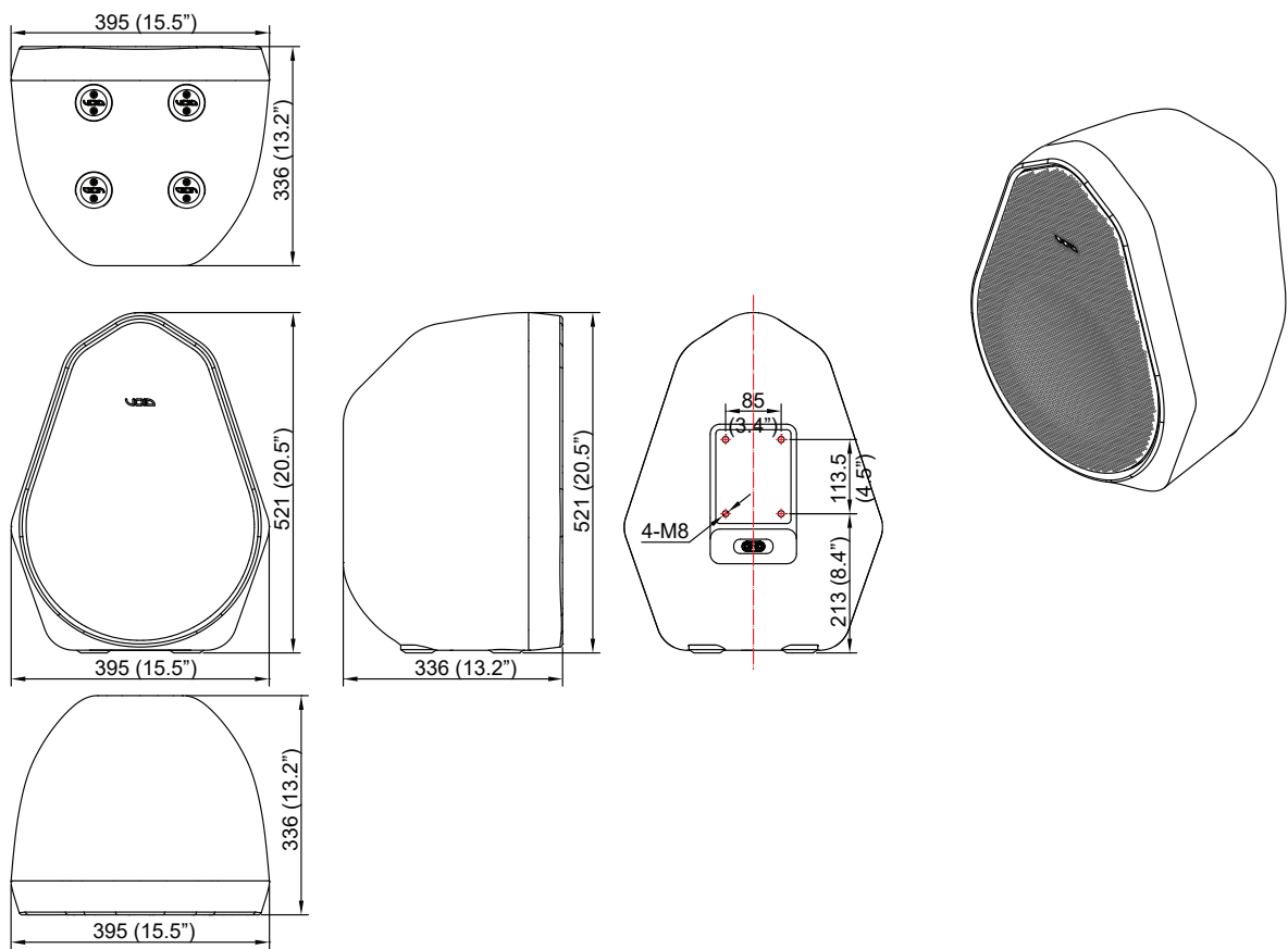
Figure 5.7: Dimensions
