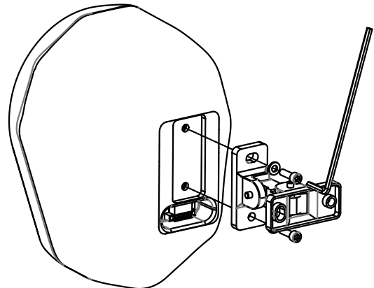
Figure 8.3: Bracket fixing
