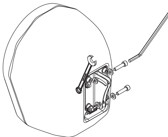
Figure 8.13: Bolt removal
