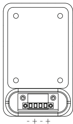
Figure 6.1: Phoenix connector
