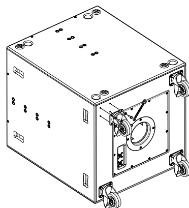
Figure 5.2: Wheel removal
