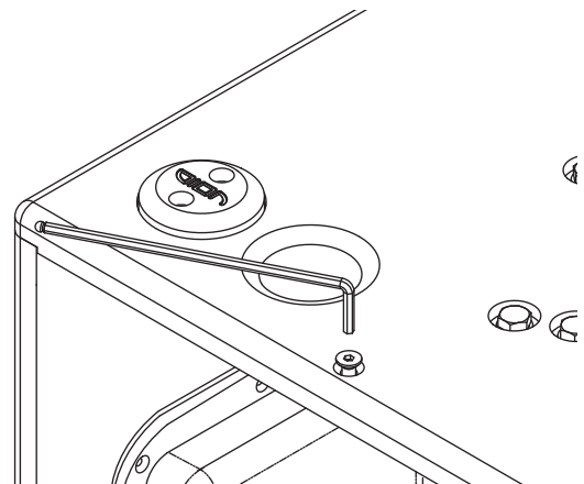
Figure 5.6: Bolt replacement
