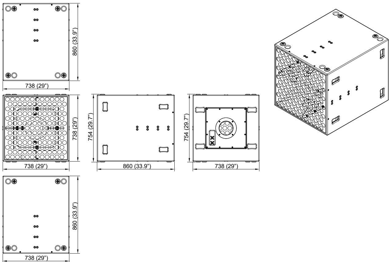
Figure 3.1: Dimensions
