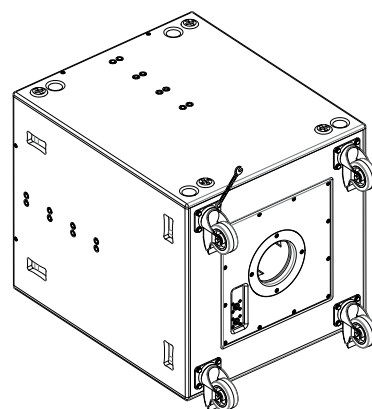
Figure 5.1: Bolt removal
