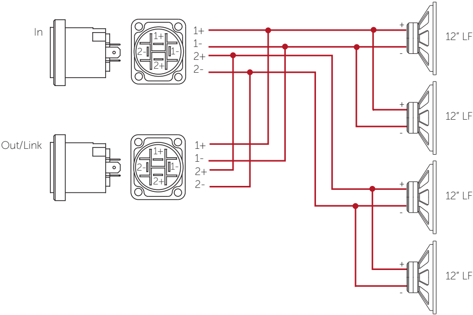
Figure 4.2: Wiring diagram
