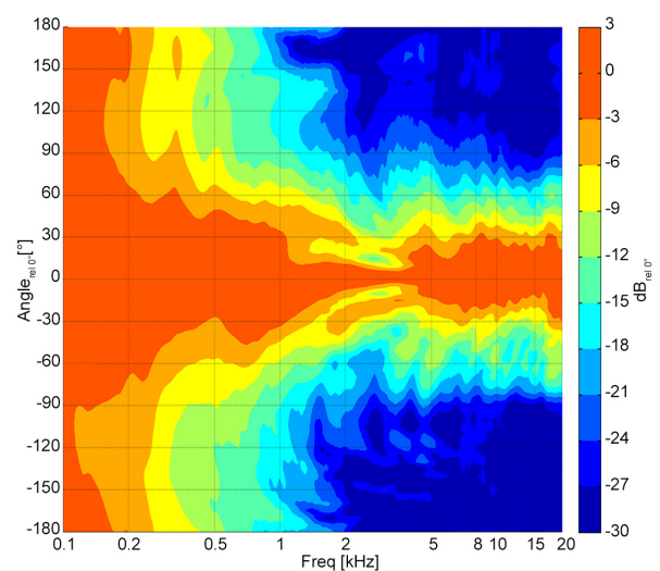
Figure A.10: Vertical directivity isobars
