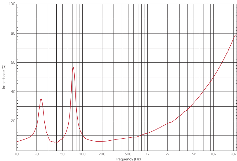
Figure A.13: Venu 115 V2 impedance graph
