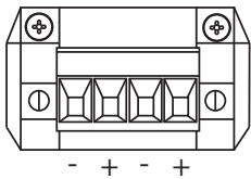
Figure 4.1: Phoenix connector polarity
