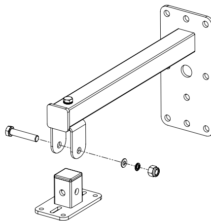
Figure 5.31: Nut removal
