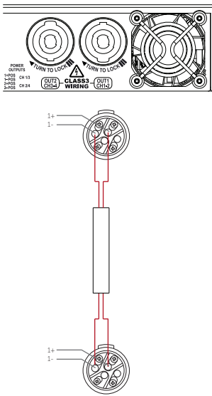
Figure 4.11: Bias Q5 speakON™ wiring
