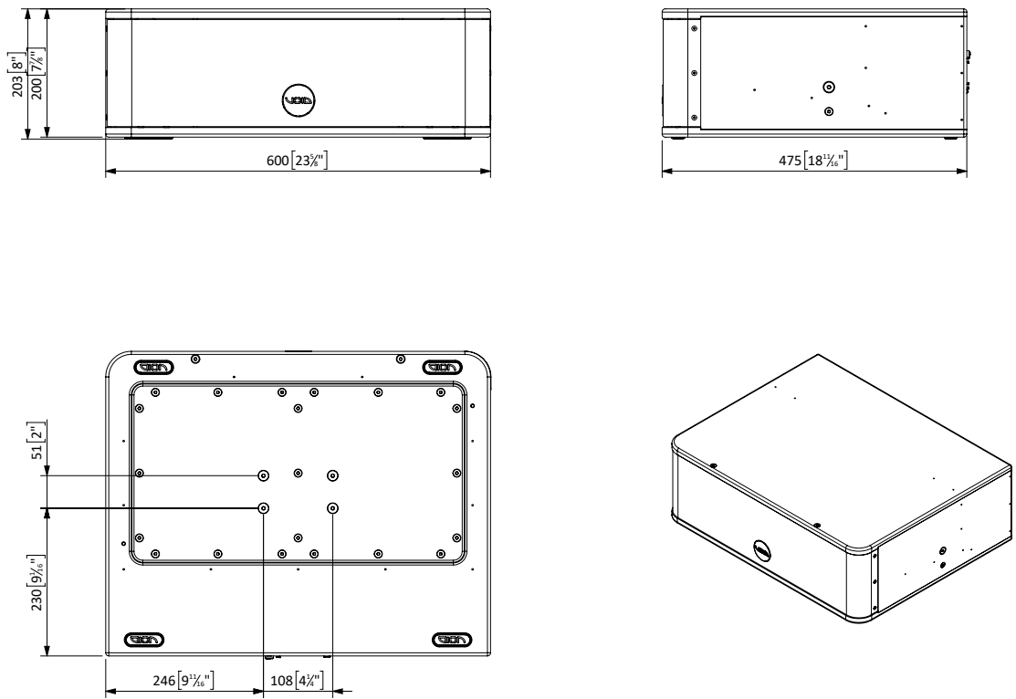
Figure 3.1: Dimensions
