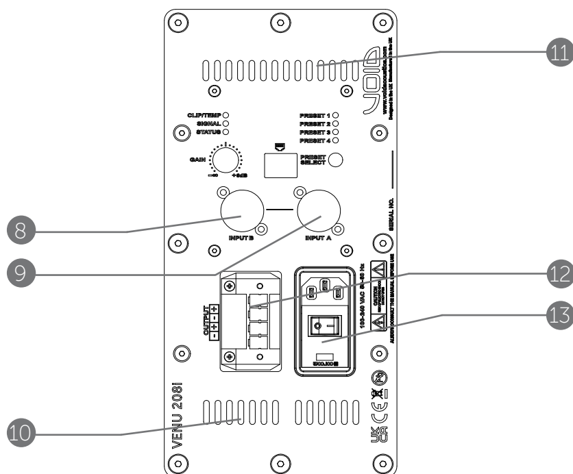
Figure 5.2: Rear panel
