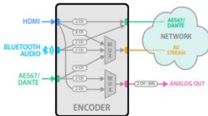
Figure 11. DuetE-WP-BT Audio Workflow Diagram
