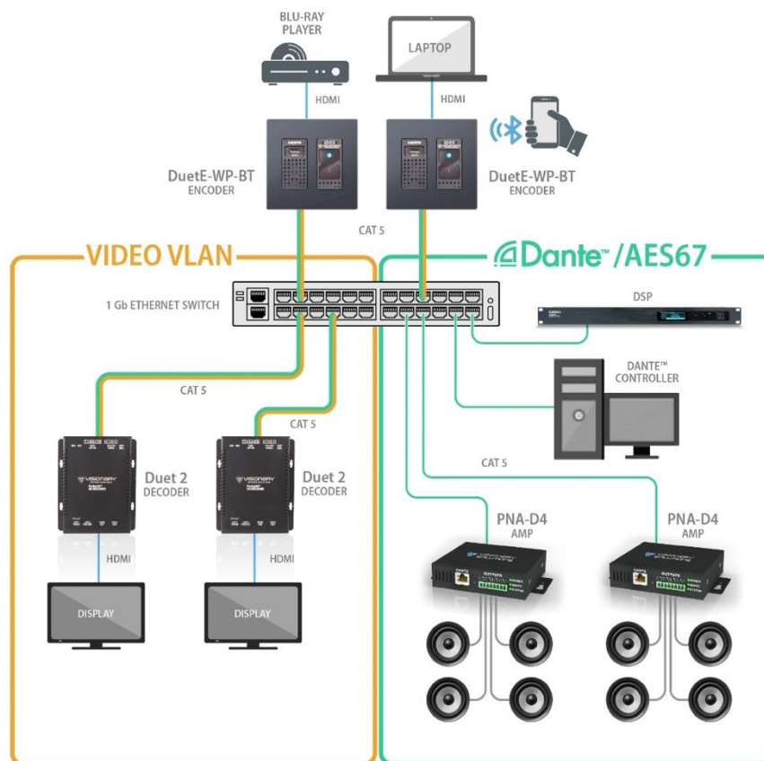
Figure 3. DuetE-WP-BT Dante™ Connection Diagram
